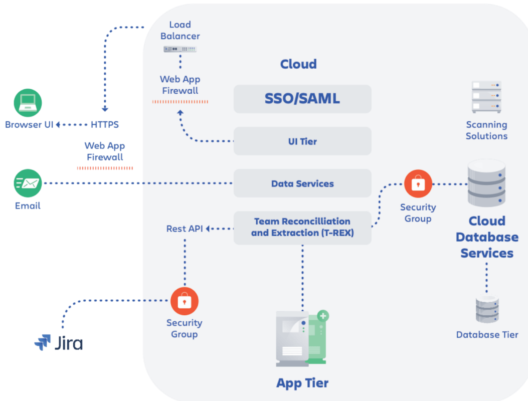
Figure 1: Jira Align Infrastructure
